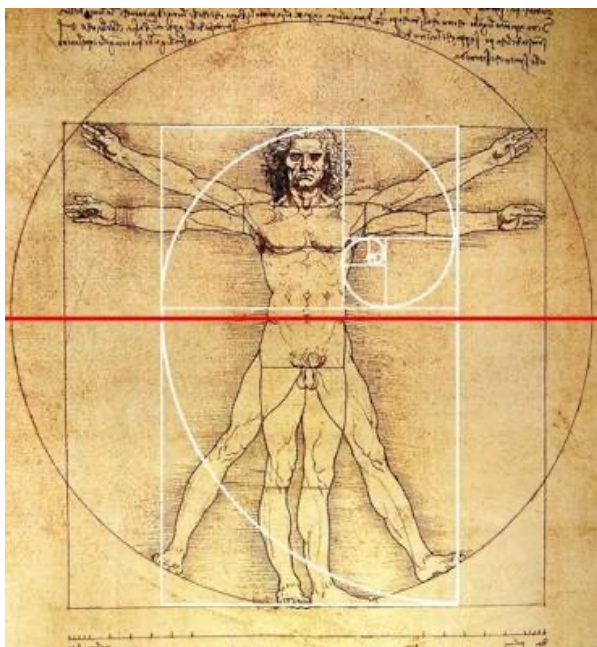
Figure 2: Fibonacci and Divine Proportion representation over the Vitruvian Man by Leonardo Da Vinci Source: Robert Grant’s and Alan Green’s discoveries
