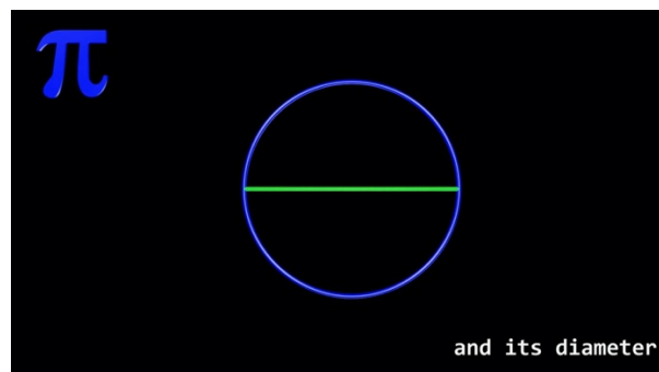
Figure 3: in a Circle of diameter 1 the size of its circumference is pi.
