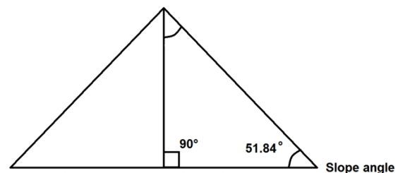
Figure 7 and 8: Illustrating the numbers pi and Phi and its correlations
