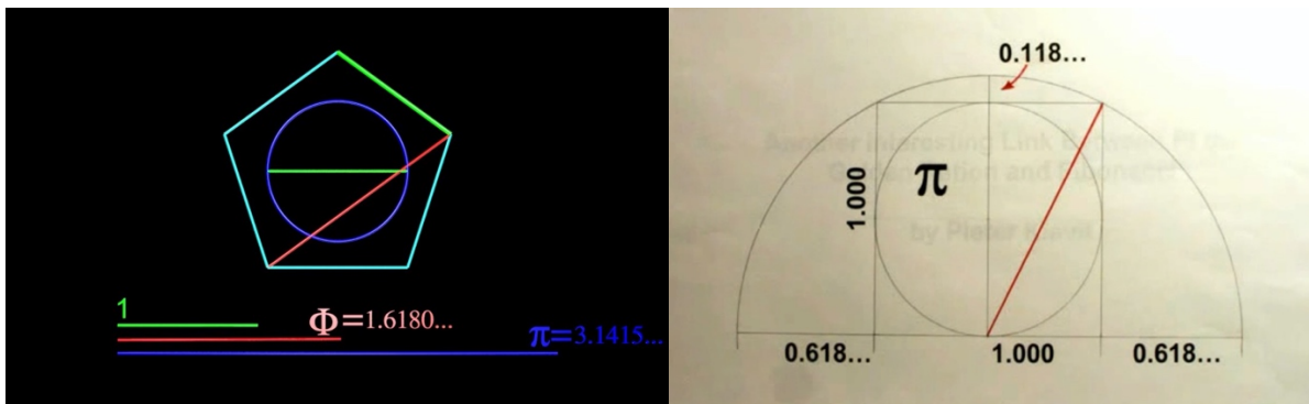
Figure 5 and 6: Illustrating the numbers pi and Phi and its correlations
