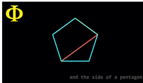
Figure 4: the length of the diagonal in a Pentagon of size 1 on its side is Phi.
